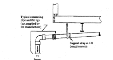
Figure A to § 3285.904 – Connection to Site Sewer.
