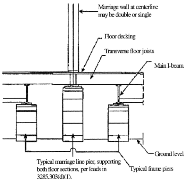
Figure C to § 3285.310 Typical Mate-Line Column and Piers.
