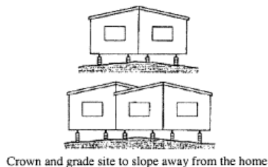
Figure to § 3285.203 - Grading and drainage.
