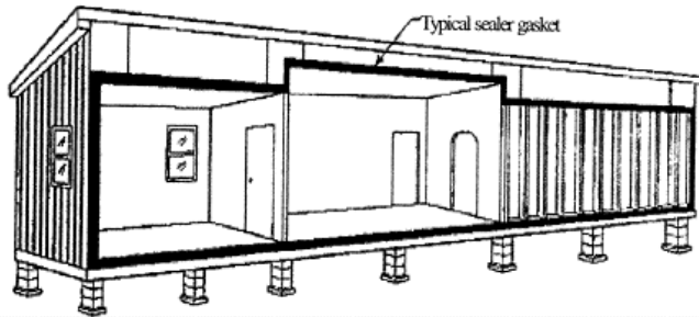
Figure B to § 3285.801 Mate-Line Gasket.
