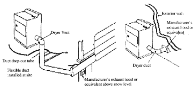
Figure A to § 3285.503 Dryer Exhaust System.
