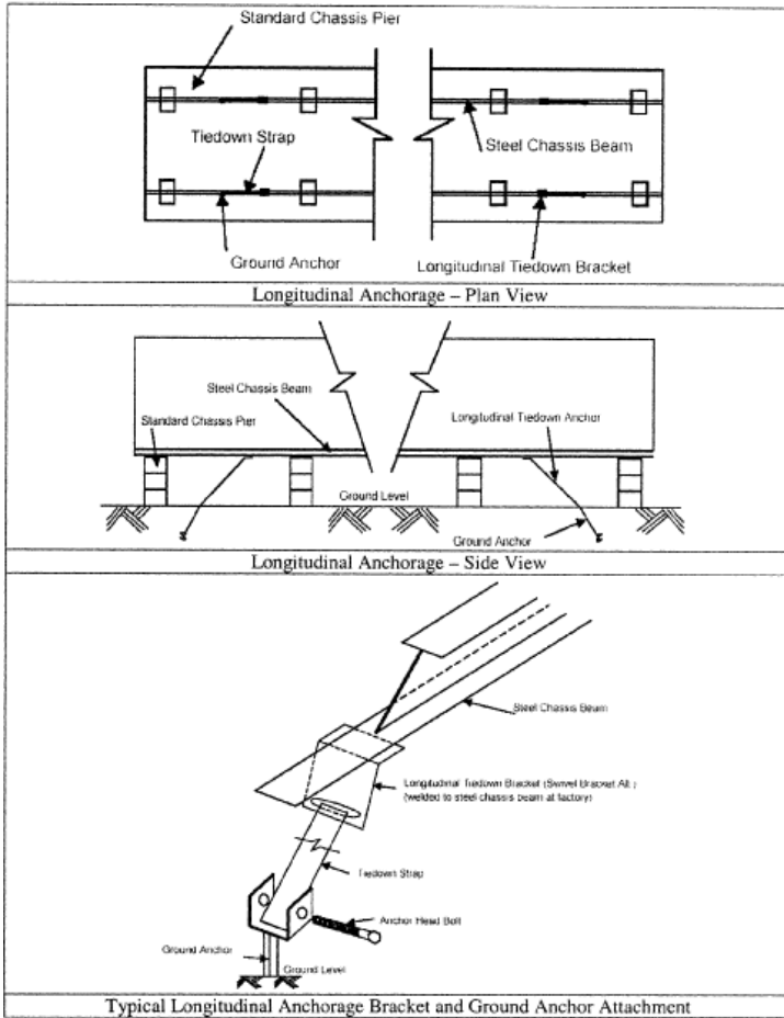
Figure C to § 3285.402 Longitudinal Anchoring
